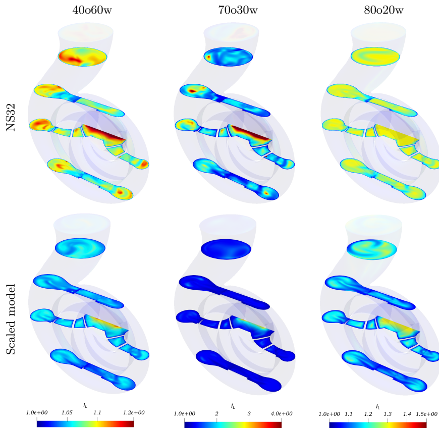
Figure 3.29: Distribution of I_L at several cross-section planes of the two pumps at different flow rates
