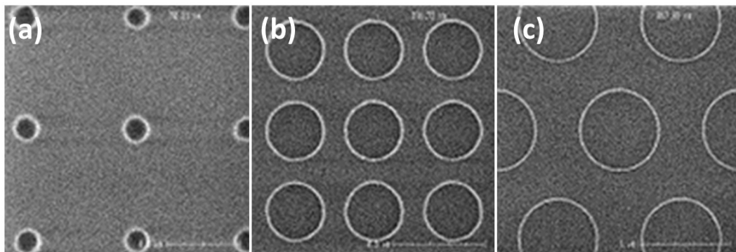
FIGURE III.9 – Images SEM de structures du Mask2 vue du dessus. (a) D = 70 \text{ nm} , \Lambda = 300 \text{ nm} ; (b) D = 317 \text{ nm} , \Lambda = 432 \text{ nm} ; (c) D = 868 \text{ nm} , \Lambda = 1374 \text{ nm} .
