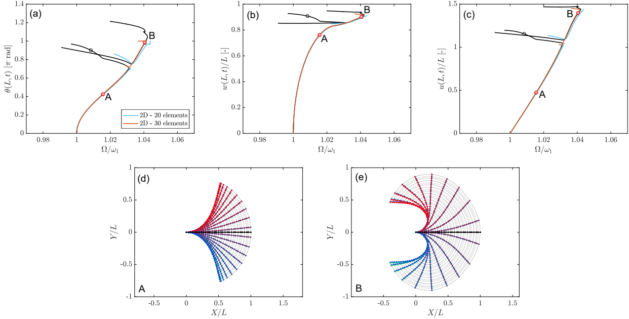
Figure 5.6: Comparison of the 2D formulations' first nonlinear mode of the cantilever beam. The backbone curve in black is a reproduction of the one shown in § 3.3.1 (2D w/ rotation matrices), (a) maximum amplitude of \theta(L,t) over one period of oscillation, (b) maximum amplitude of the transverse displacement w(L,t)/L , (c) maximum amplitude of the axial displacement u(L,t)/L , (d) deformed shape at point A, representing 20 snapshots over one half period of motion, overlaid onto the deformed shapes of § 3.3.1, (e) deformed shape at point B.
