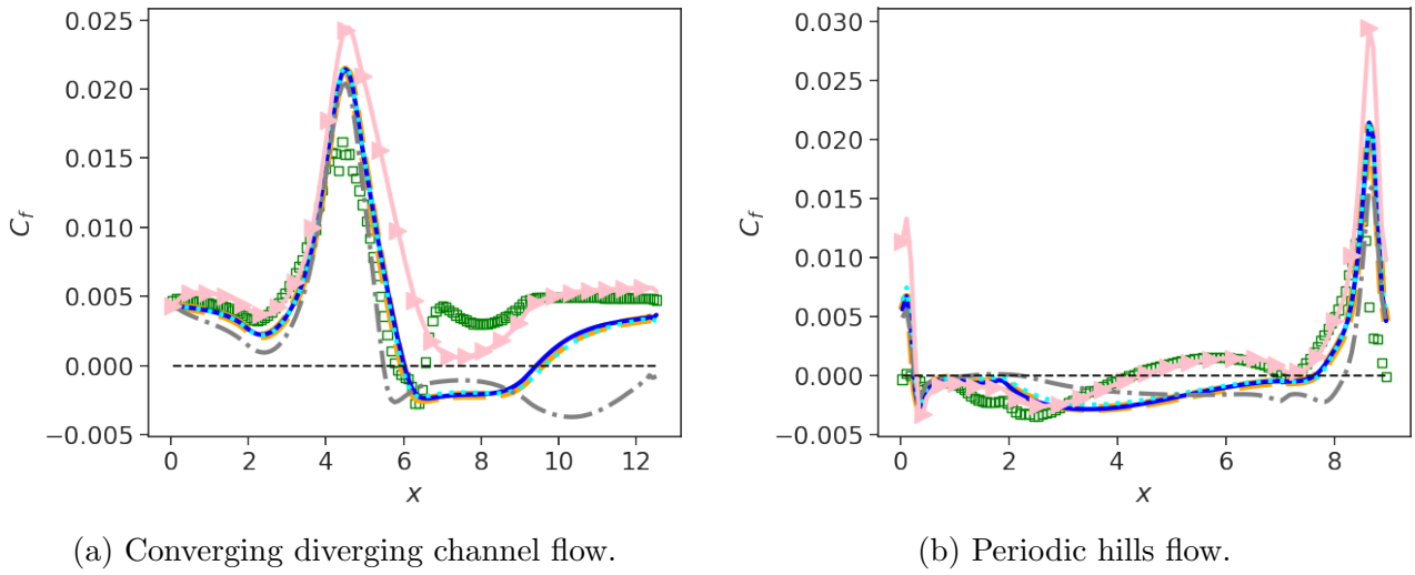
Figure 5.4: Skin-friction distributions along the bottom wall - various SBL-SpaRTA models. \mathbf{M}^{(ZPG)} (---), \mathbf{M}^{(CHAN)} (—), \mathbf{M}^{(APG)} (····), \mathbf{M}^{(ANSJ)} (---), \mathbf{M}^{(SEP)} (→), High-fidelity data (□).
