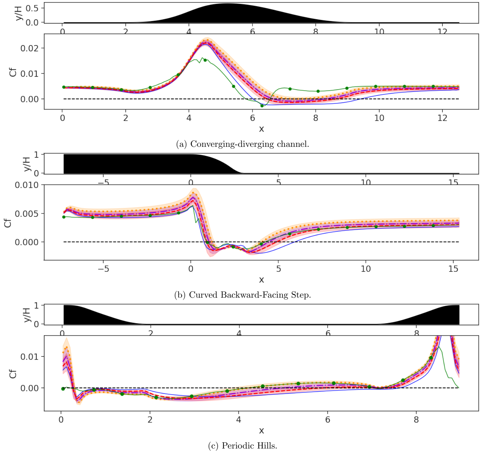
Figure 4.7: Friction coefficient distributions along the bottom wall: baseline k - \omega SST ( \text{—} ), LES ( \text{—}\bullet\text{—} ), and SBL models with \pm 3 standard deviation confidence intervals: \mathbf{M}^{(1)} ( \cdots , \square ), \mathbf{M}^{(2)} ( -\cdot- , \square ) and \mathbf{M}^{(3)} ( -\cdot- , \square ).
