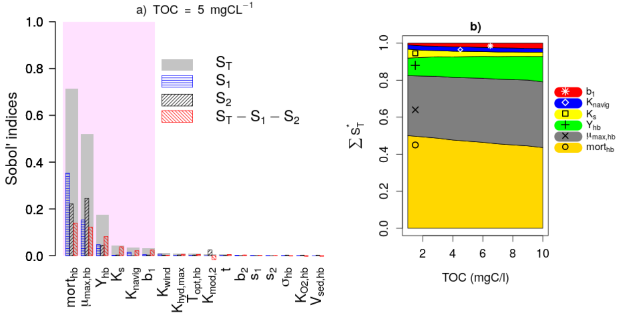
Figure 3.4: Sobol SA results of first SA: All parameters (a) Sobol SA results for TOC = 5 mgCL -1 ; (b) Evolution of the normalized total sensitivity indices of the influential parameters with TOC
