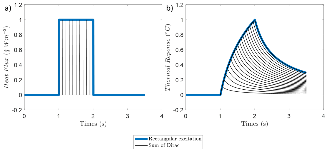
Figure 5.14: Decomposition of heat sources: (a) heat flux function of time and (b) thermal response of the system.
