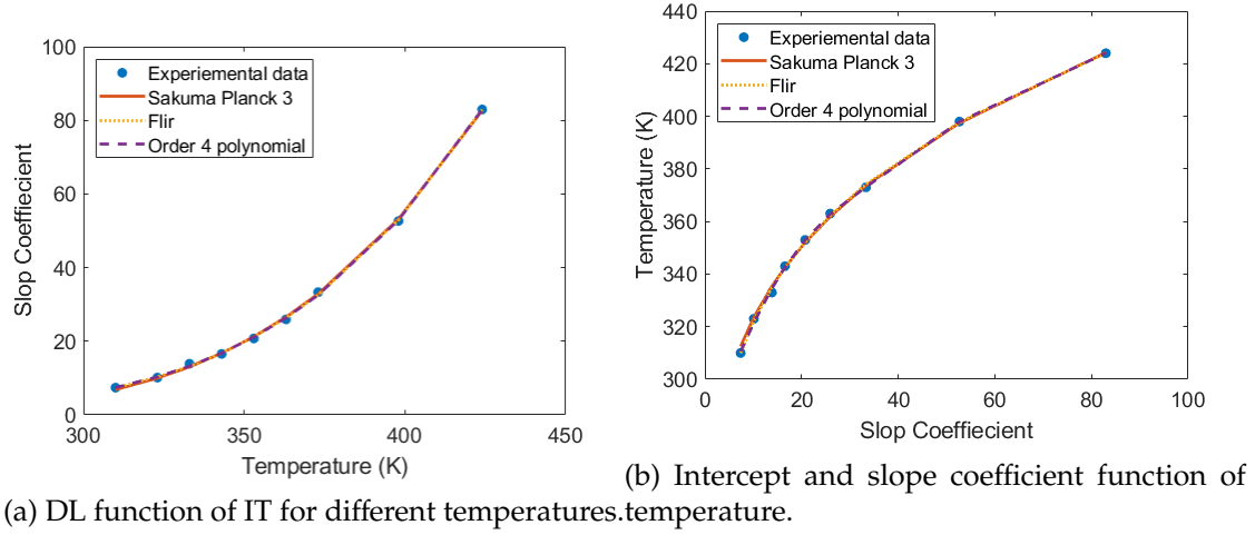
Figure 4.16: Slope coefficient fitting for InSb low-temperature calibration.
