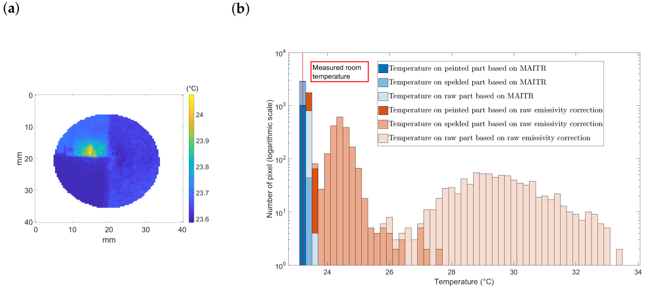
Figure 4.35: Sample temperature distribution (°C): (a) temperature map; (b) histogram of temperatures for the ATR and emissivity correction methods. The room temperature is measured as 23.2 °C.
