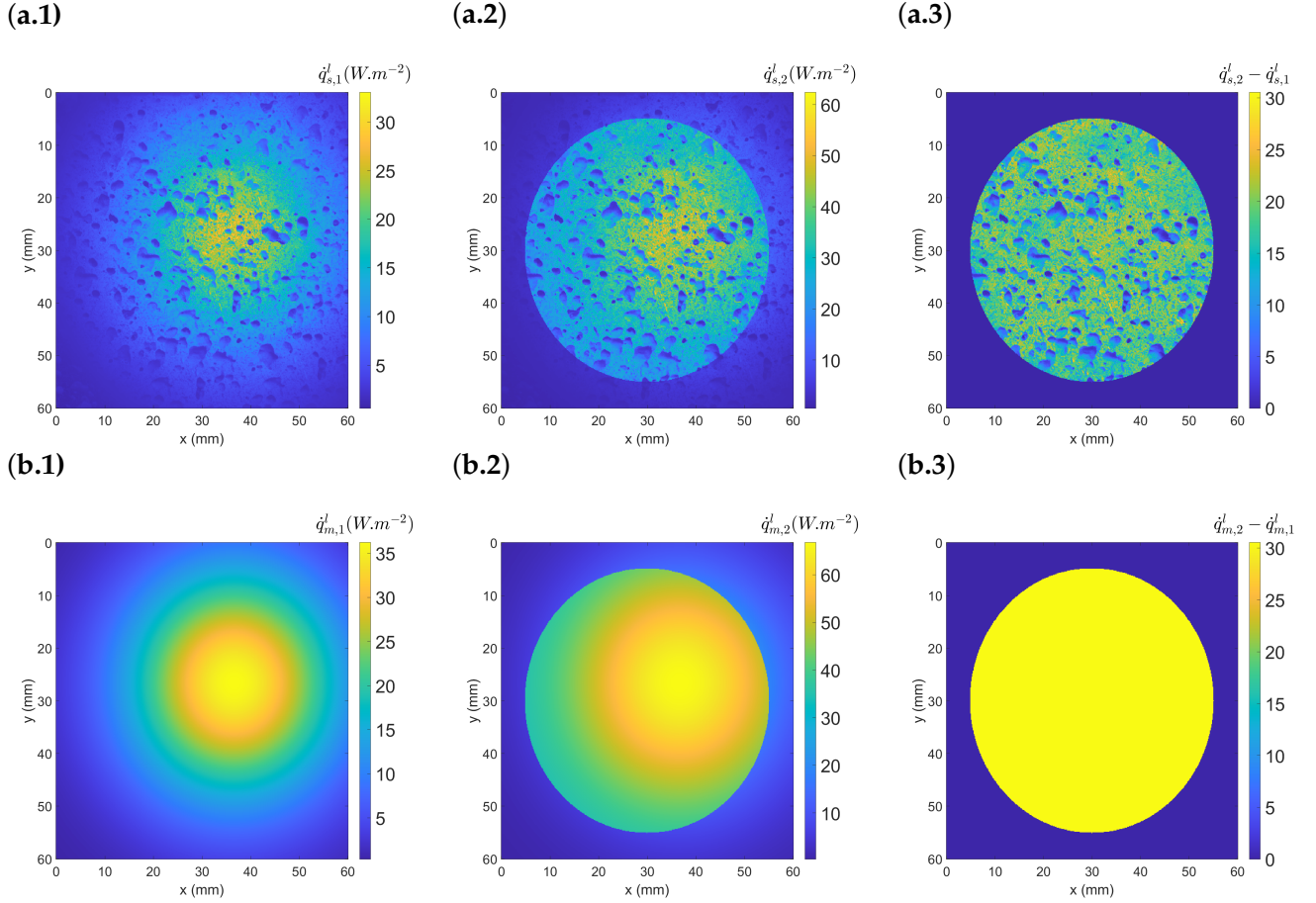
Figure 4.24: Simulated camera response (step 2 of ATR) for a heterogeneous sample (a) and a reference mirror (b): (a.1) radiative image from the sample \dot{q}_{s,1}^l ; (a.2) radiative image from the illuminated sample \dot{q}_{s,2}^l ; (a.3) difference between both images \dot{q}_{s,2}^l - \dot{q}_{s,1}^l ; (b.1) radiative image from the mirror \dot{q}_{m,1}^l ; (b.2) radiative image from the illuminated mirror \dot{q}_{m,2}^l ; (b.3) difference between both images \dot{q}_{m,2}^l - \dot{q}_{m,1}^l .
