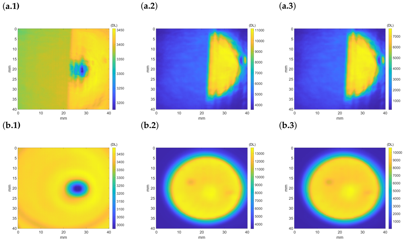
Figure 4.27: Camera measurements (step 2 of ATR) on the (a) stainless steel sample, where the left side is the rough surface and the right is the laser-polished surface, and (b) for the reference mirror. (a.1) raw sample measurement \dot{q}_{s,1} ; (a.2) illuminated sample \dot{q}_{s,2} ; (a.3) difference \dot{q}_{s,2} - \dot{q}_{s,1} ; (b.1) raw mirror measurement \dot{q}_{m,1} ; (b.2) illuminated mirror \dot{q}_{m,2} ; (b.3) difference \dot{q}_{m,2} - \dot{q}_{m,1} .
