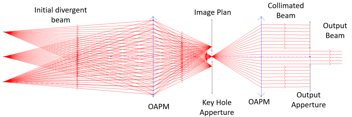
Figure 3.10: Optical schema of the collimation optical assembly.
