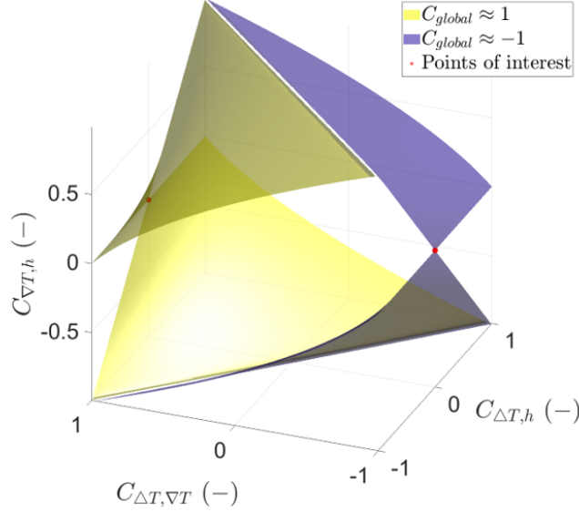
Figure 5.8: Behaviour of the C_{global} function of (a) C_{\nabla T, \Delta T} , (b) C_{\Delta T, h} and (c) C_{\nabla T, h} .
