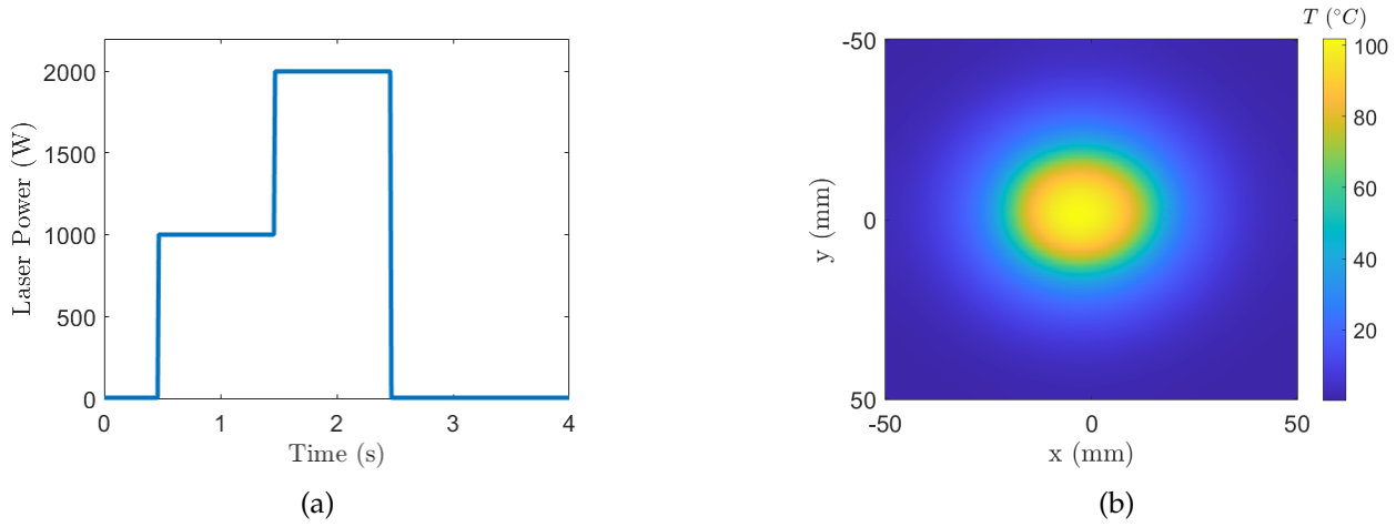
Figure 6.34: a) Excitation temporal profile for the calibration and (b) image of the maximum measured temperature.
