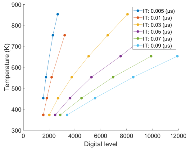
Figure 6.19: Camera calibration curves for multiple ITs.
