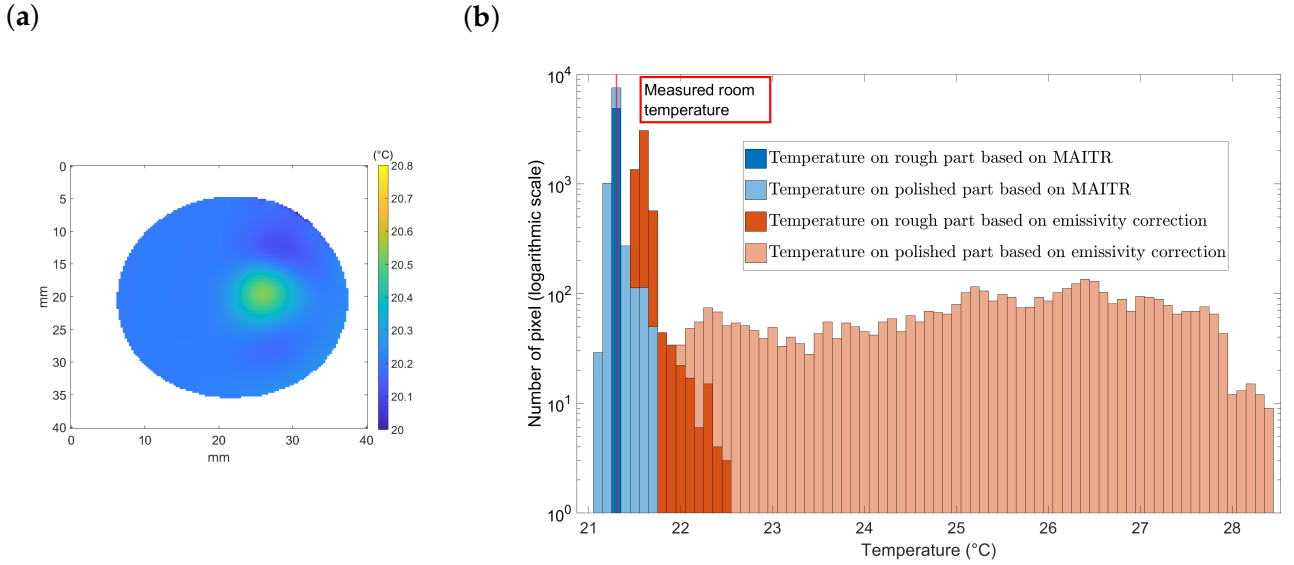
Figure 4.30: Sample temperature distribution (°C): (a) temperature map; (b) histogram of temperatures for ATR and emissivity correction methods. The room temperature is measured to be 21.3 °C.
