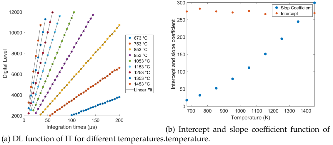
Figure 4.12: Linear fit description of the InSb high-temperature calibration.
