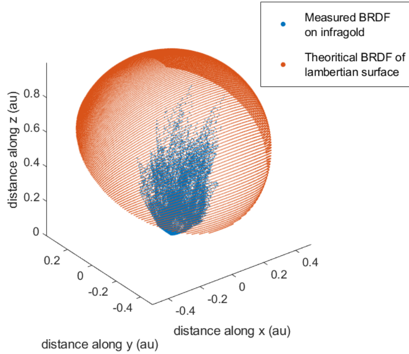
Figure 3.24: Normalised measured BRDFs of the mirror.
