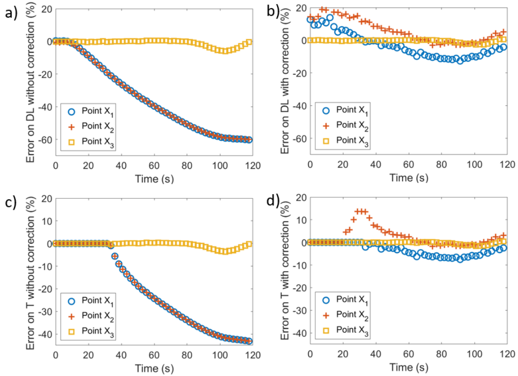
Figure 6.24: Error obtain though the application of ATR method: (a) DL error without correction, (b) DL error with correction, (c) temperature error without correction, (d) temperature error with correction.
