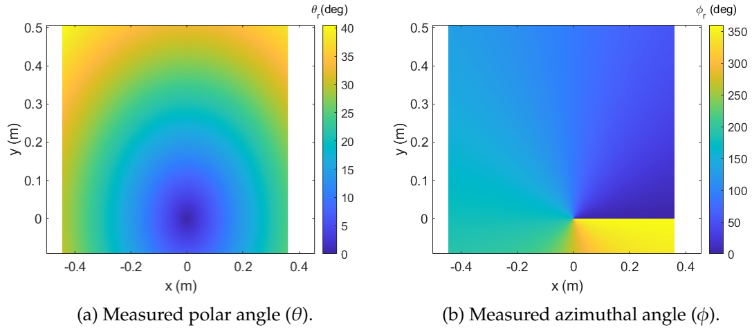
Figure 6.13: Illustration of measured polar coordinates.
