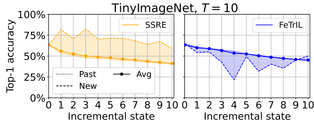
Fig. 4.5.: Top-1 incremental accuracy per state for past and new classes for TinyImageNet, with T = 10 incremental states for FeTrIL 1 and SSRE, the best compared method. An ideal method would provide high accuracy, but also similar performance for past and new classes. The accuracy of past and new classes is globally closer for FeTrIL 1 , which indicates that our method provides a better stability-plasticity balance than SSRE. Overall accuracy is better for FeTrIL 1 in Figure 4.3 because the contribution of new classes in each state diminishes during the CIL process.
