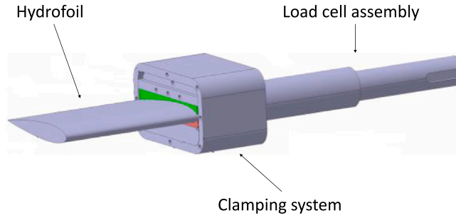
Fig. 2. Sketch of the hydrofoil mounting system.
