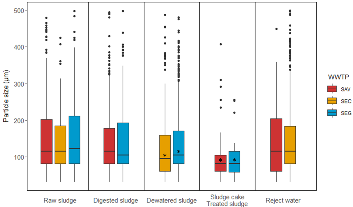
Figure 3-4: Size distribution of MPs (25-500 \mu\text{m} ) in different sludge types and reject water from three studied WWTPs. The box (IQR=Q3-Q1) presents the 50 % of the central size dataset. The line inside the box (Q2) presents the median particle size. The upper whisker shows the data range up to Q3+1.5*IQR . The lower whisker shows the data range down to Q1-1.5*IQR . In which, Q1-First quartile, Q2-Second quartile, Q3-Third quartile and IQR-Interquartile range. Outliers of the dataset are located outside the whiskers and shown in black dots. The asterisks show a significant change in median size of MPs in one sludge type compared to particles in raw sludge from the same plant with p\text{-value} < 0.05 .
