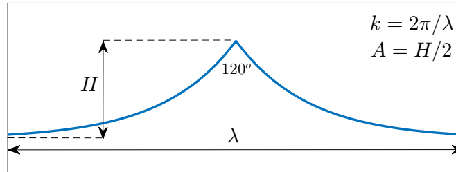
Figure 1.5: Limiting Stokes wave in deep water.
