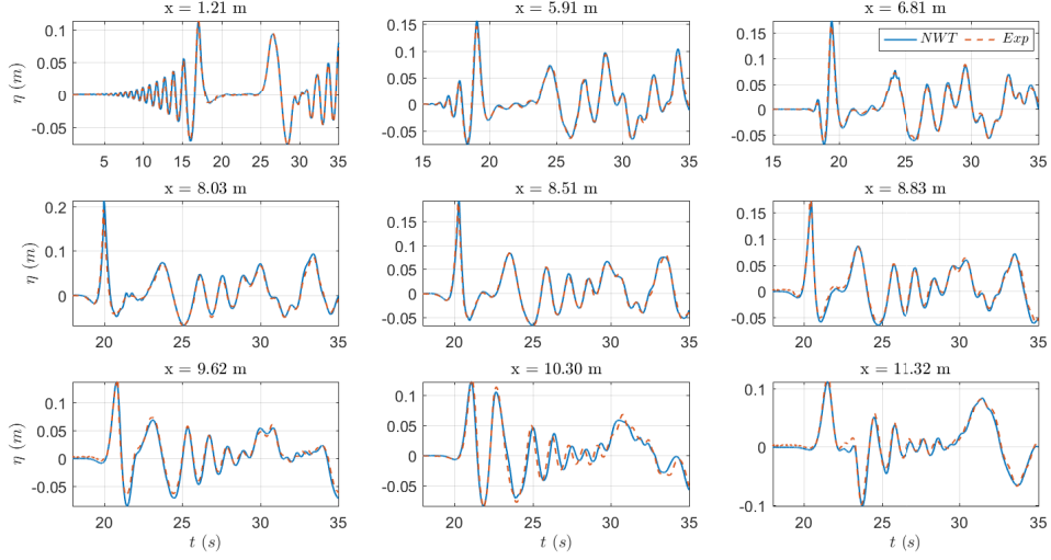
Figure 3.7: Time series comparison of the free surface elevation from the experiments (dashed line) and the NWT (solid line) at the 9 wave gauge locations for the test case F1 ( H = 0.2377 m, x_f = 7.8 m). Wave breaking crest seen at x \in [7.78, 8.60] m, and t \in [19.85, 20.36] s as modeled with the initiation and termination criteria.
