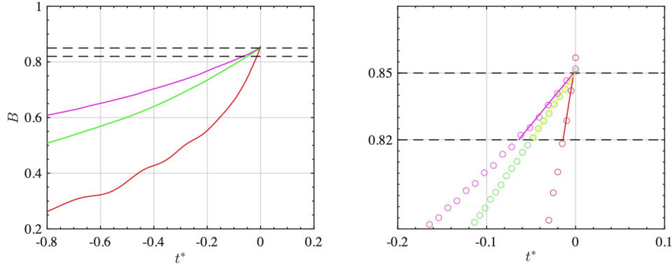
Figure 2.2: Evolution of B = u/c in simulations with the Misthyc model as a function of non-dimensional time t^* = (t - t_b)/T_b ( t_b denotes the time of breaking onset when B = B_{th} = 0.85 ), for periodic: (i) plunging breaking waves propagating over a bar, from Beji & Battjes (1993) (BB-regular, red); (ii) spilling breaking waves propagating over a plane slope, from Hansen & Svendsen (1979) (HS, magenta); and shoaling and spilling breaking waves propagating over a plane slope, from Ting & Kirby (1994) (TK, green).
