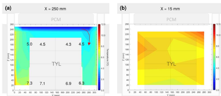
Figure 2.14 Air temperature field on (a) the middle ( x = 250 mm) and (b) the lateral ( x = 15 mm) planes of the box with PCM on the lid. Values indicate the time-averaged core and surface temperatures of the test packs.
