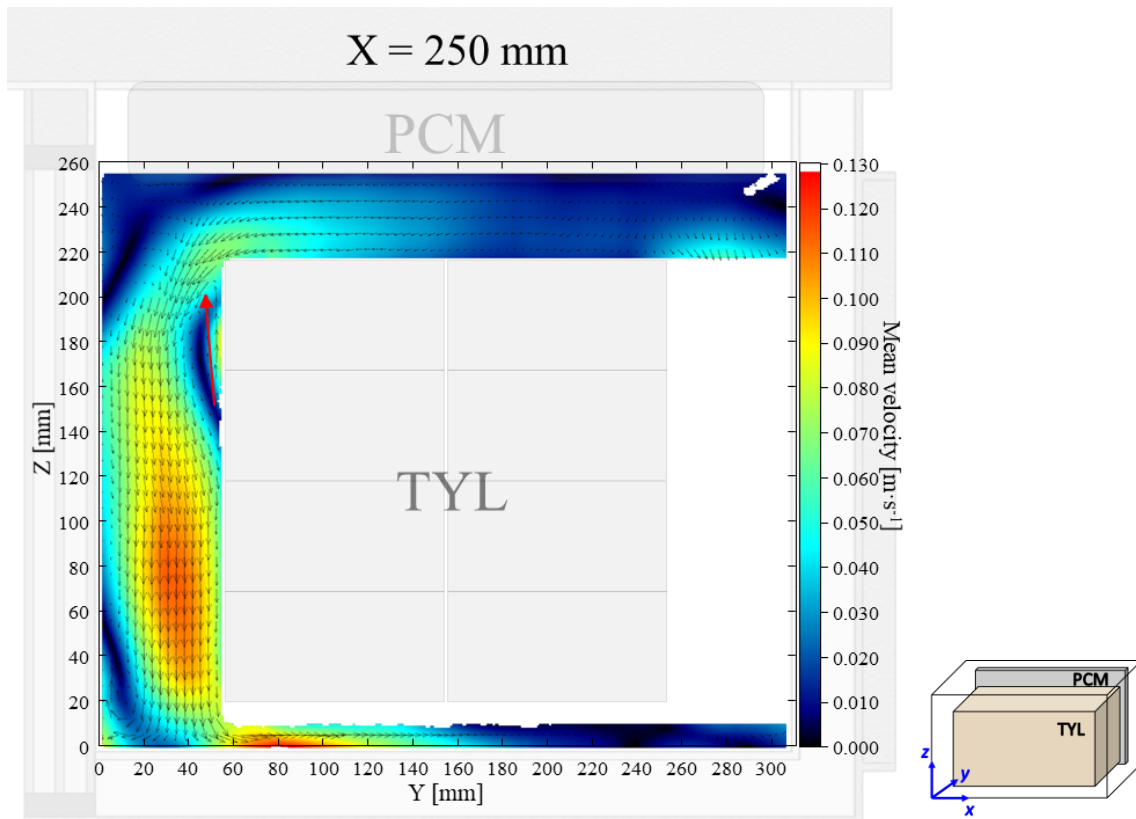
Figure 7: Air velocity field on the middle plane in a loaded horizontal box with PCM at the top under 30^\circ\text{C} ambient, product initial temperature = 4^\circ\text{C} with 20 mm gap below. White area on the right represents the unmeasurable zone because of the inaccessibility of laser sheet.
