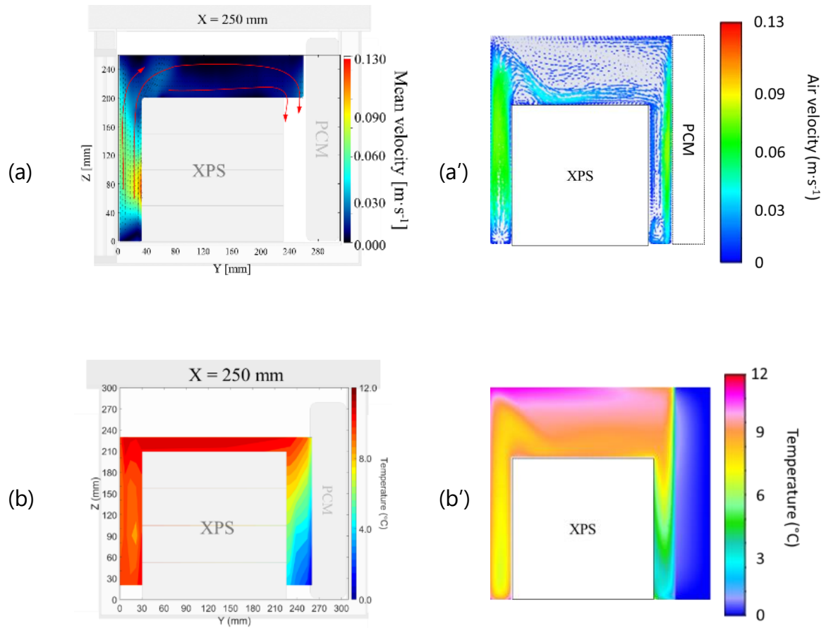
Figure 3.14 (a) Experimental air velocity field and (b) experimental temperature field on the middle plane of a box loaded with XPS with PCM on a sidewall. (a') and (b') are corresponding numerical results
