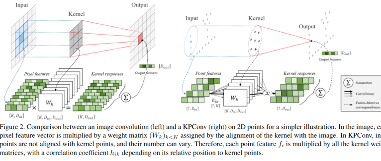
FIGURE 2.6 – Illustration de KPConv, extrait de [37].
