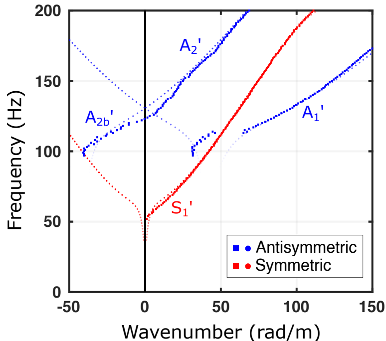
FIGURE 1.23: Dispersion curves of in-plane modes in the clamped strip ( 2h' = 50.6 mm) – Experimental (squares) and theoretical (circles) dispersion curves (the more transparent the more attenuated). The A_2' Dirac cone (linear crossing of the k=0 axis) and backward A_{2b}' modes (negative wavenumbers) are unambiguously evidenced.
