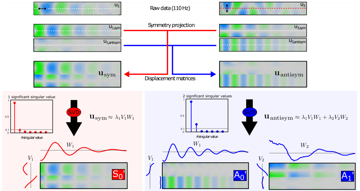
FIGURE 1.17: Mode separation via Singular Value Decomposition (SVD) – At 110 Hz, in-plane displacement components u_1 and u_3 (top left) are projected onto their symmetrical and anti-symmetrical parts (top right). Data are then concatenated into a single complex matrix \mathbf{u}_{\text{sym}} (resp. \mathbf{u}_{\text{antisym}} ) on which the SVD is directly applied. After extracting most significant modes (singular values above a 10% threshold), we obtain one symmetrical ( S'_0 ) and two anti-symmetrical ( A'_0 and A'_1 ) modes.
