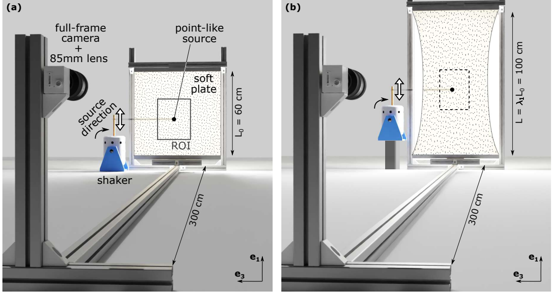
FIGURE 2.1: Experimental setup to measure velocities in a deformed plate – (a) A thin plate of Ecoflex00-30, with dimensions 60 cm x 3 mm x 60 cm in directions x_1, x_2, x_3 , is held in a vertical position and clamped to a frame on its top and bottom edges. Sinusoidal vibrations in the (x_1, x_3) -plane are generated by a shaker and displacements are extracted using a CCD camera located 3 m away from the plate. (b) Same experimental configuration but the frame is adjusted to impose large deformations, reaching stretch ratio \lambda_1 > 2 along the vertical axis.
