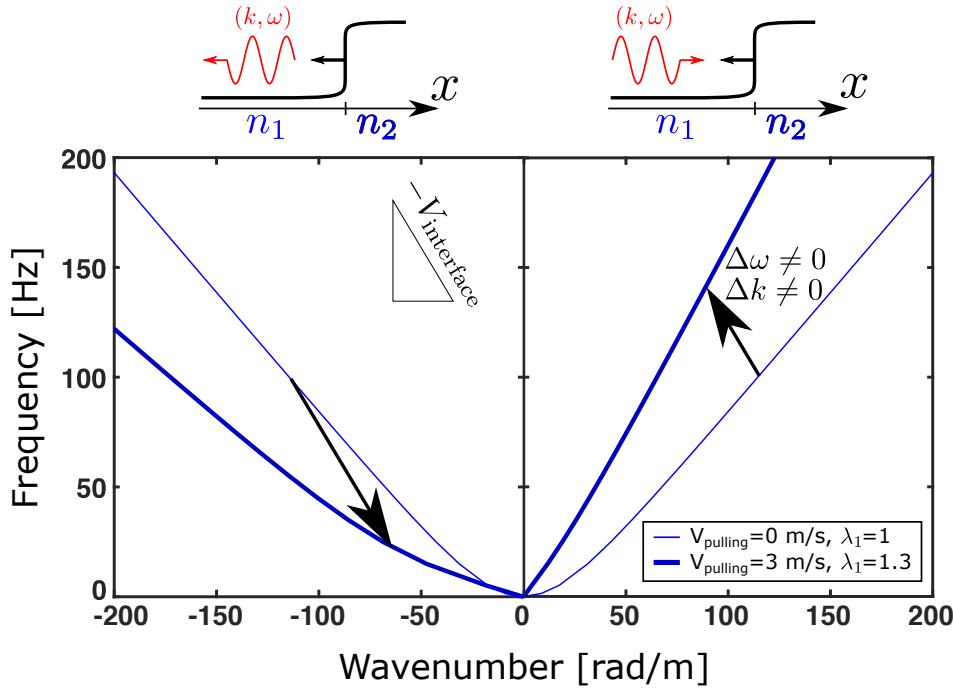
FIGURE 5.9: Crossing a space-time interface – Using dispersion curves of the in-plane flexural mode A'_0 in figure 5.8, the crossing of a moving interface is illustrated by a tilted ( \Delta\omega/\Delta k = -V_{\text{interface}} ) jump from a dispersion curve to another. Depending on the interface propagation direction, different conversions are expected.
