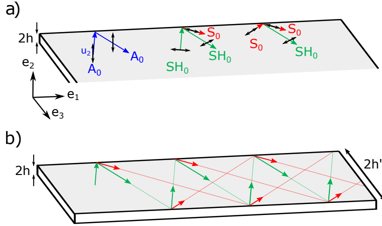
FIGURE 1.13: Mode coupling in a strip – (a) Reflection of A_0 on the edge only generates A_0 while S_0 and SH_0 modes couple. (b) Multiple reflections lead to S_0 and SH_0 in-plane mode coupling in a similar manner to shear and longitudinal waves couple in an infinite plate, as in figure 1.3.
