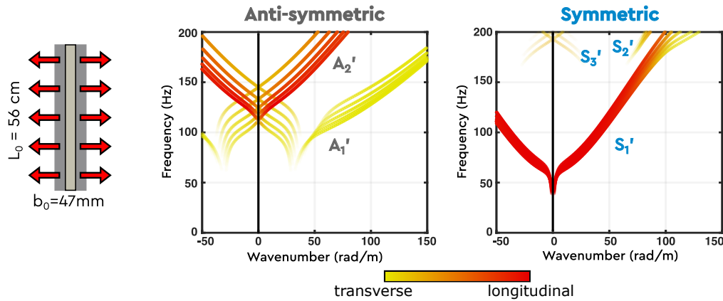
FIGURE 3.9: Role of the polarization for a fixed strip – Theoretical dispersion curves for the fixed strip subjected to a planar stress. The color indicates the dominant polarization (yellow = transverse, red = longitudinal).
