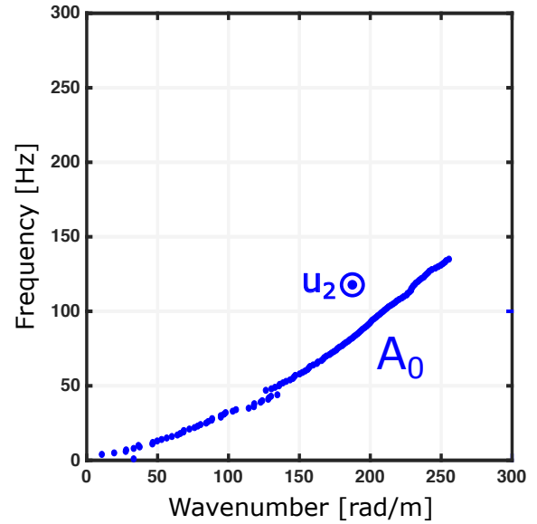
FIGURE 1.12: Experimental dispersion curves of the flexural mode in a 3-mm-thick soft plate – The quadratic behaviour of A_0 , first anti-symmetric Lamb mode, or flexural mode, in a plate is retrieved.
