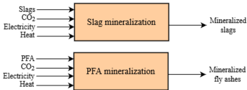
Figure 33: Input/output flows in CO 2 mineralization processes.
