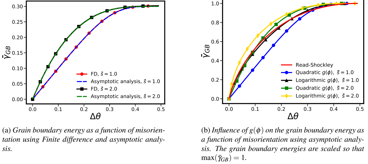
Figure 3.9: Grain boundary-misorientation curves for different values of \bar{s} and \bar{\alpha} = 0.3, \bar{\varepsilon} = 2 .
