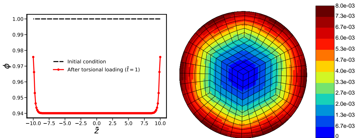
(a) Profile of \phi along the vertical axis of the rod.
