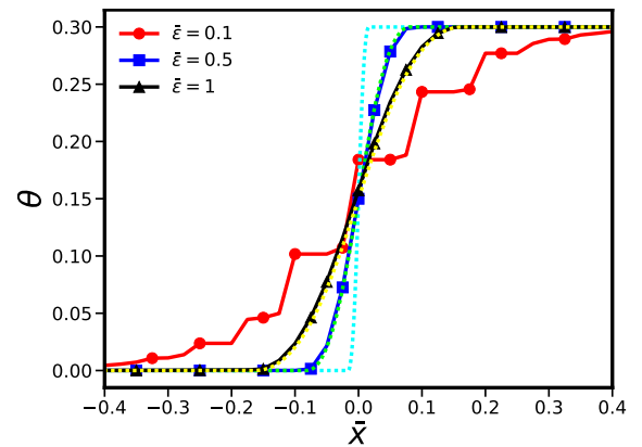
(b) Profiles of \theta for different \bar{\epsilon} and fixed \bar{\alpha}, \bar{s}
