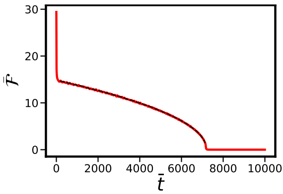
(a) Total dimensionless energy as a function of time.
