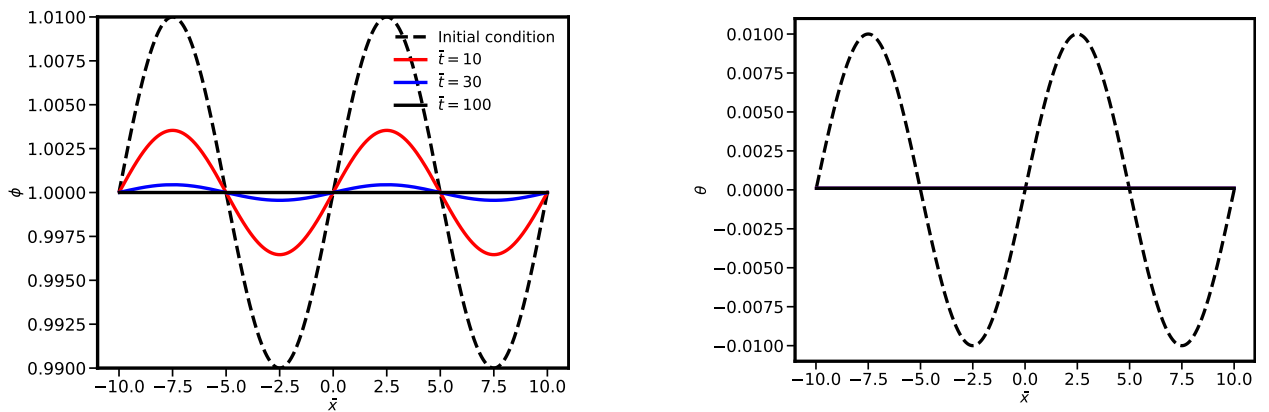
Figure 4.1: Profiles of \phi and \theta for \gamma = 10 , \xi = 10 in the quadratic regime and \phi_0 = 1 , \theta_0 = 0 .
