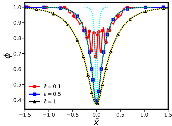
(a) Profiles of \phi for different \bar{\epsilon} and fixed \bar{\alpha}, \bar{s}
