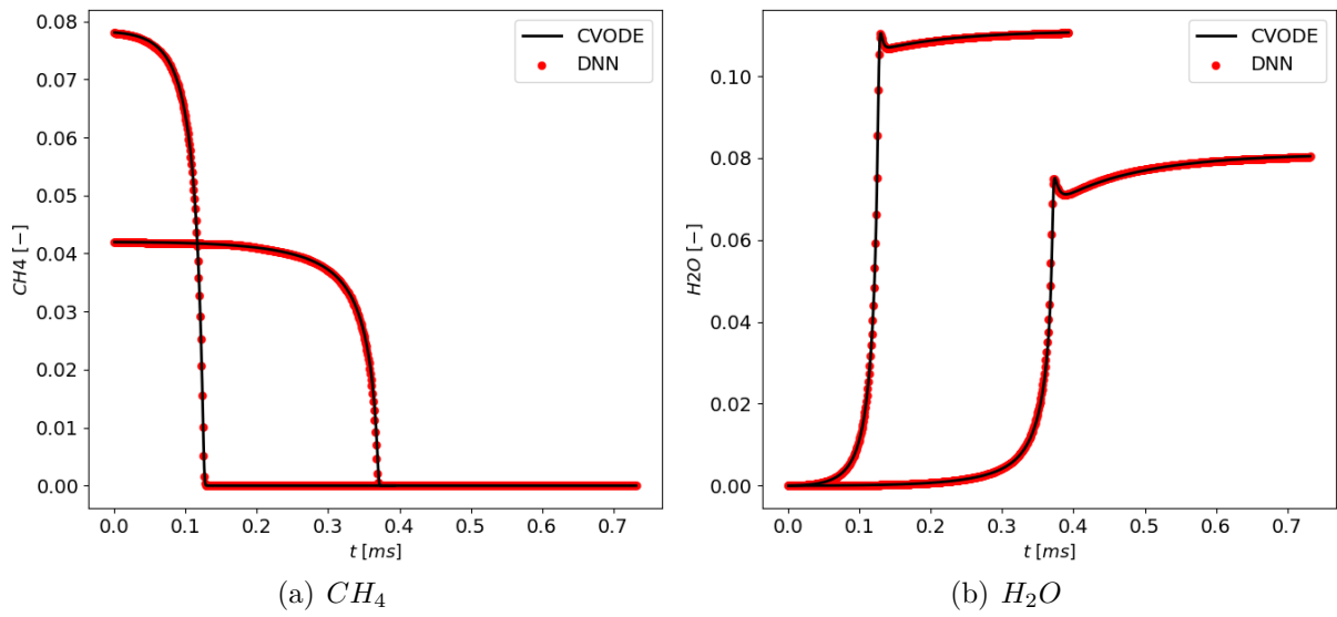
Figure 3.17: Continuous inference simulation for CH_4/air case with 2 trajectories: T_{01} = 1620.0K, \phi_1 = 0.75 and T_{02} = 1790.0K, \phi_2 = 1.45 .
