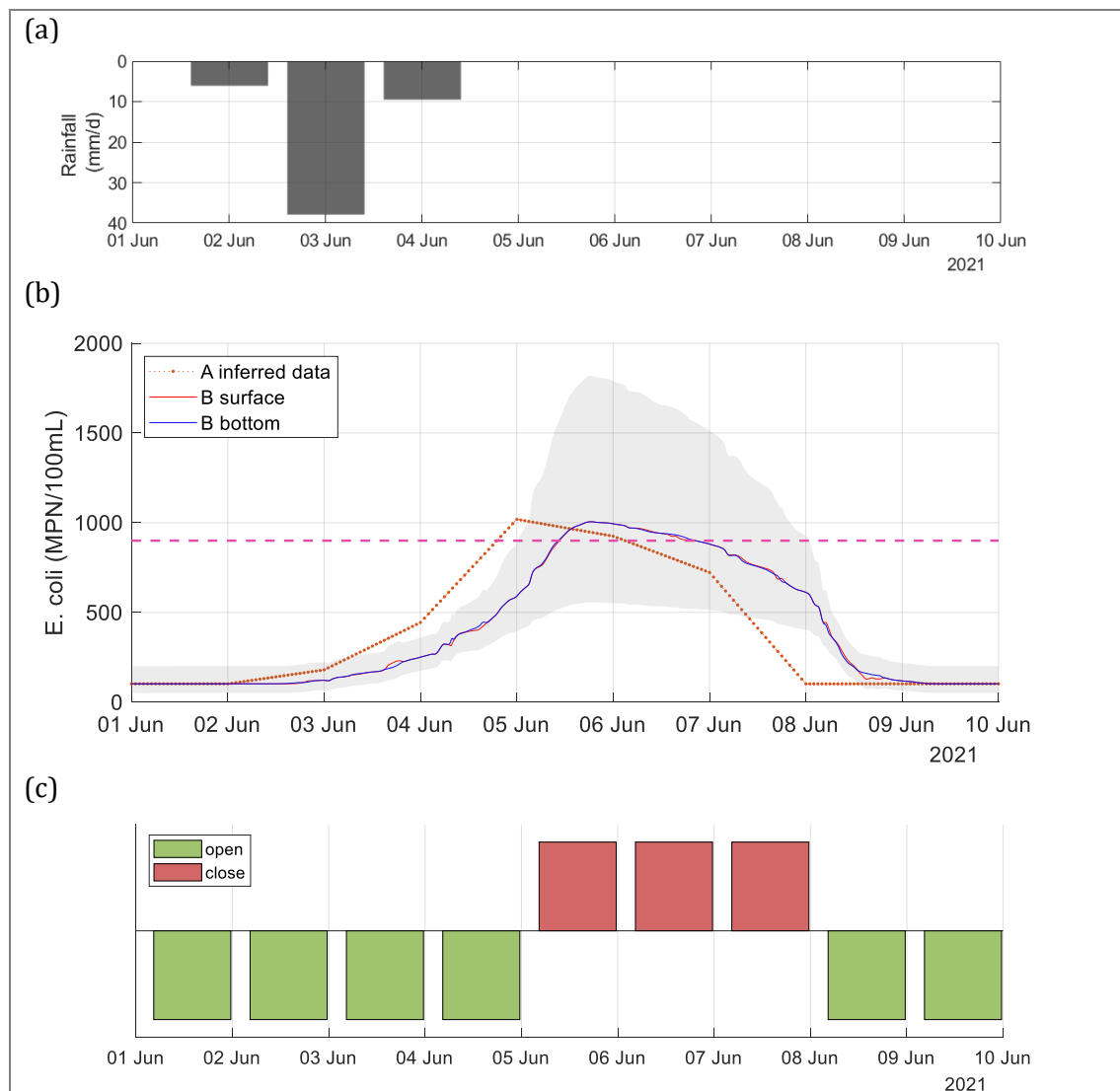
Figure 4.86. June 2021: (a) Daily rainfall at Le Bourget station. (b) E. coli simulation results at point B (bathing area) on surface layer (red), bottom layer (blue) and the confidence interval (grey), with the bathing threshold of 900 MPN.100mL -1 (dashed line). (c) Indication of opening (green) and closure (red) days of the bathing area, according to simulation results. Data from 01 to 10/06/2021.
