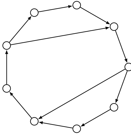
Figure 3.2: An odd directed cycle having two chords in the same direction of odd length.
