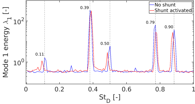
Figure 5.17: Energy spectra of the first SPOD mode for the non-activated and activated shunt configuration at U_0 = 4.4 \text{ m.s}^{-1} ( Re_c = 3.74 \times 10^5 ).
