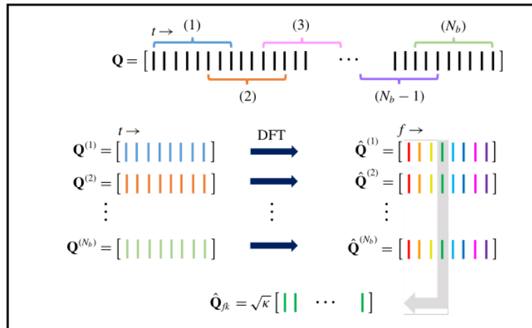
Figure 2.14: Schematic presentation of the Welch’s method for estimating SPOD modes. Figure by Towne et al. [21].
