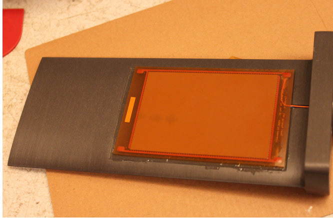
Figure 2.6: Image of the truncated hydrofoil. The MFC transducer is visible and was not covered by epoxy at this stage of the manufacturing.
