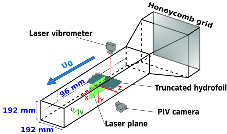
Figure 2.2: Test-section of the IRENav hydrodynamic tunnel.
