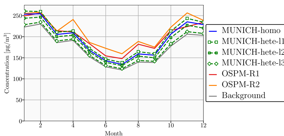
(a) CO
