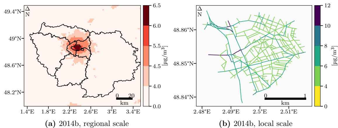
Figure 4.C.6: Annual average concentrations of OM for the baseline simulation 2014b at the regional scale (left panel) and local scale (right panel) in \mu g m^{-3} .
