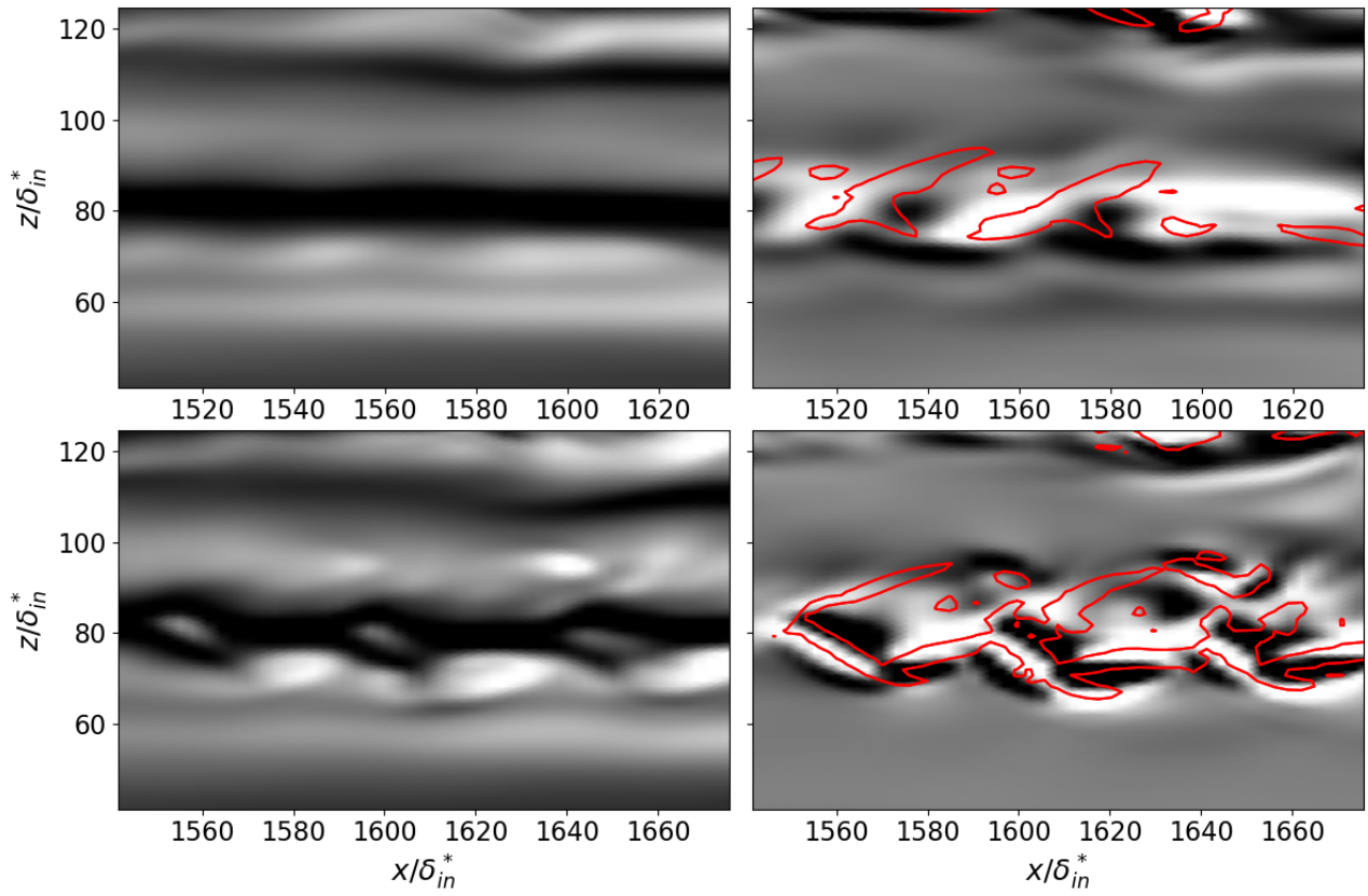
Figure 4.26: Observation of a varicose-like breakdown in the high L_f -low T_u case over two successive times (top and bottom). Streamwise fluctuations (left, u' = \pm 0.25U_\infty from black to white) and wall-normal velocity fluctuations (right, v' = \pm 0.01U_\infty (top) and \pm 0.03U_\infty (bottom) from black to white). Isolines of the Q-criterion projected around the wall-normal position of the plane are plotted in red.
