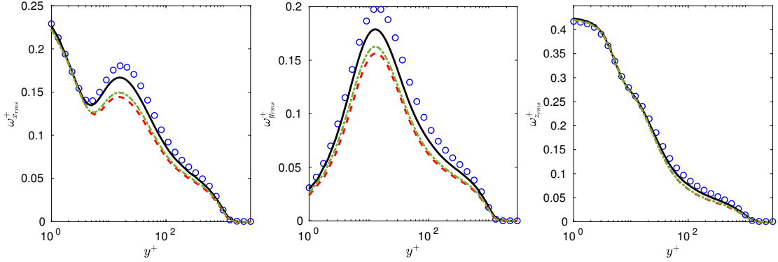
Figure 3.23: R.m.s. of vorticity fluctuation components for x -, y - and z -directions: DNS (—); LES-expl (- -); LES-IRS (- · -); DNS of Schlatter & Örlü [227] (○).
