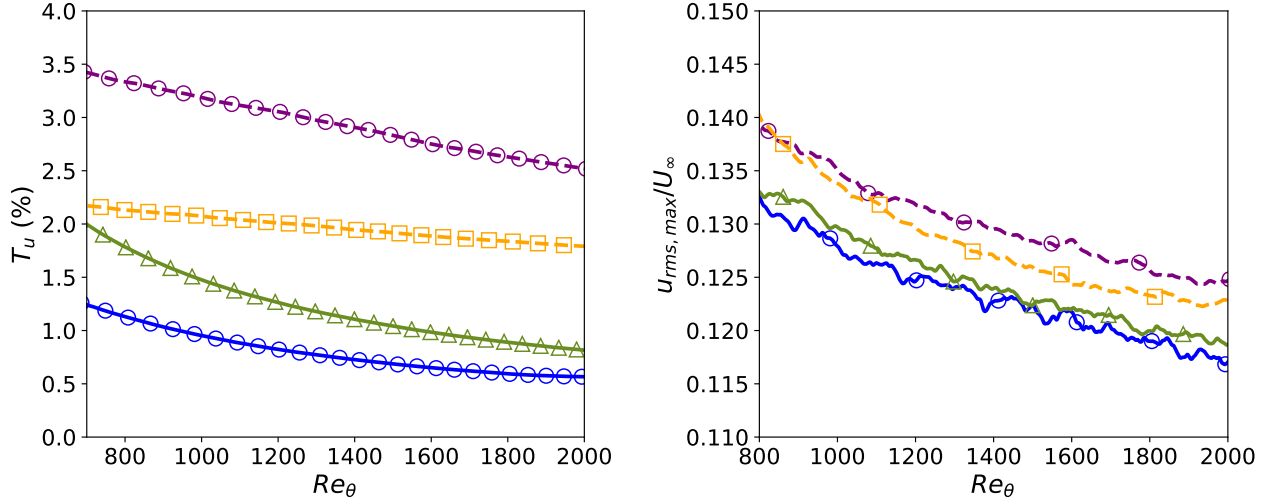
Figure 4.36: Evolution of the FST intensity (left) and u_{rms,max}/U_\infty in the BL (right) for the different Novec cases in the TBL region: low L_f (—), high L_f (---) and T_u = 2.5\% ( \square ), 4\% ( \circ ) and 6.6\% ( \triangle ).
