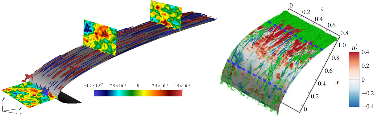
Figure 1.5: Left: Snapshot of streamwise velocity perturbation u'_t in a DNS of streaks growth around a NACA0008 wing under FST (from Faúndez Alarcón et al. [60]). Right: Snapshot of u'_t in a well-resolved LES of transition around LS89 turbine under relatively high FST intensity (from Zhao & Sandberg [59]).
