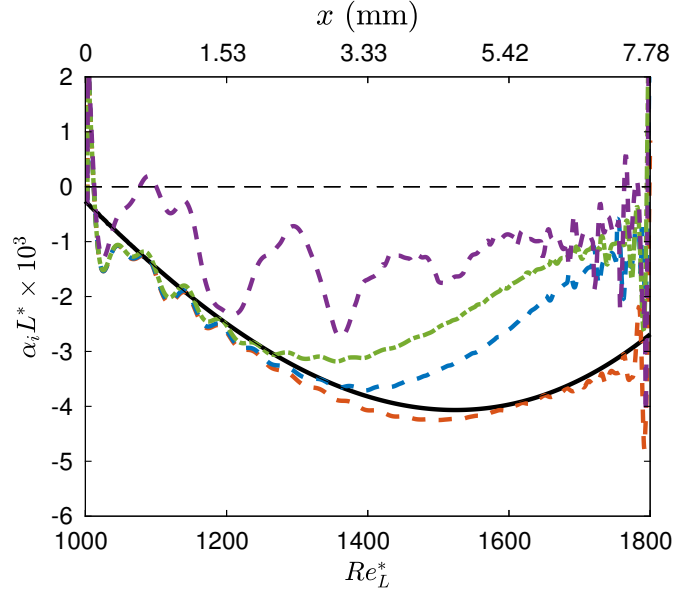
Figure 3.5: Growth rate from DNS of 2D TS waves with various amplitudes ( \varepsilon_0/U_\infty = 10^{-4} - - -; 5 \times 10^{-4} - - -; 10^{-3} - . - .; 5 \times 10^{-3} - - -) compared to LST (—).
