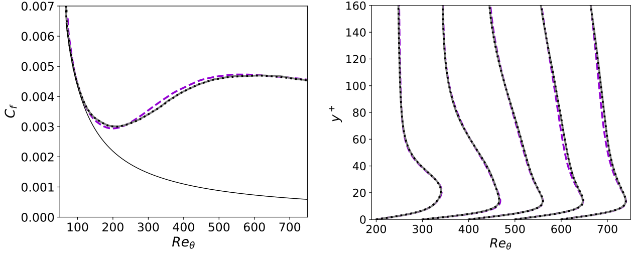
Figure C.3: Friction coefficient evolution (left) and streamwise fluctuating velocity 50 \times \frac{u_{rms}}{u_\tau} + Re_\theta (right) for the high L_f -high T_u Air M=0.9 configuration with LES resolution with N=100 modes (---) and DNS resolution with N=100 (.....) and N=116 (—) RFM modes.
