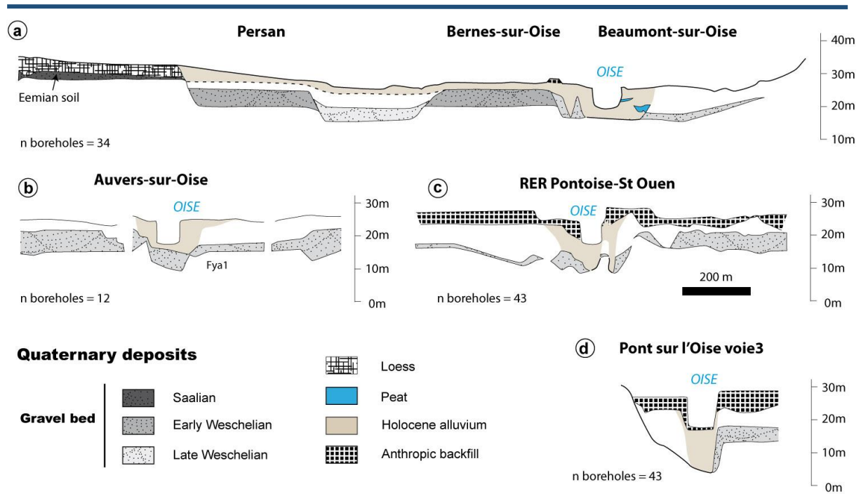
Figure 7.2. Cross-sections in the alluvium of the lower part of the Oise valley (after Krier, 2004). See Figure 1 for location. Based on existing and recent (Blaser et al., 2015; Chourio Camacho, this thesis Chapter 3) dating of alluvial sediments (Table 7.1), the extension of Holocene sediment has been largely reduced compared to the initial interpretation by Krier (2004).
