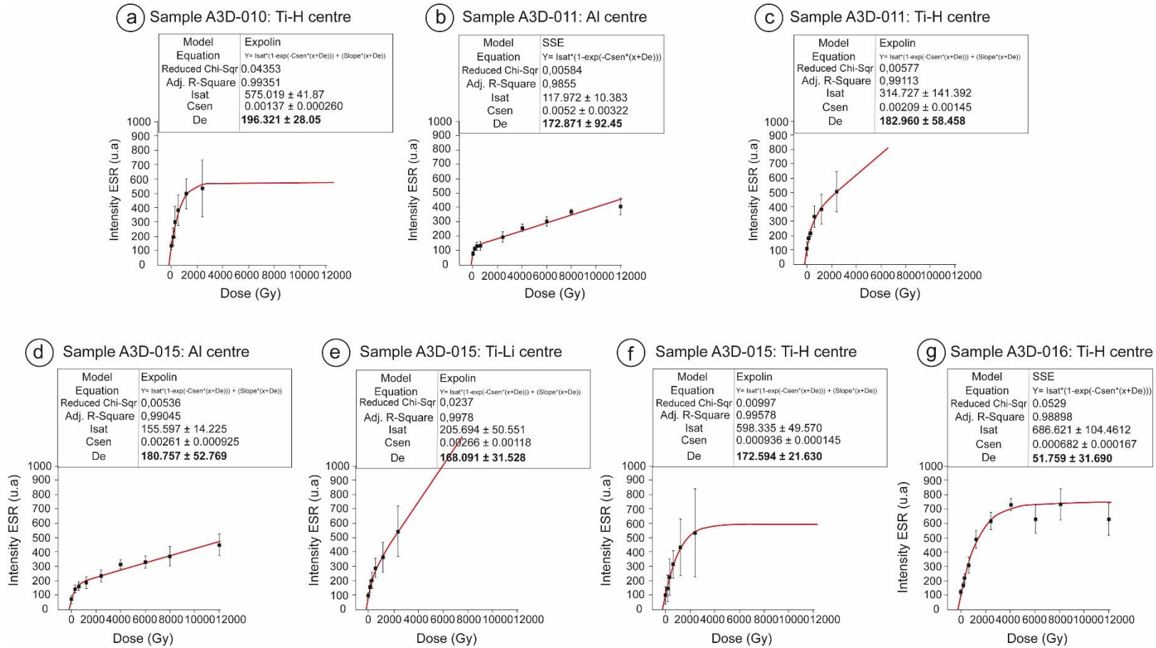
Figure E.1.2. Dose response curves derived from the measurements of the (a) Ti-H centre (sample A3D-010), (b) Al centre (sample A3D-11), (c) Ti-H centre (sample A3D-11), (d) Al centre (sample A3D-015), (e) Ti-Li centre (sample A3D-015), (f) Ti-H centre (sample A3D-015) and (g) Ti-H centre (sample A3D-016). Fitting was performed using the SSE or Expolin functions.
