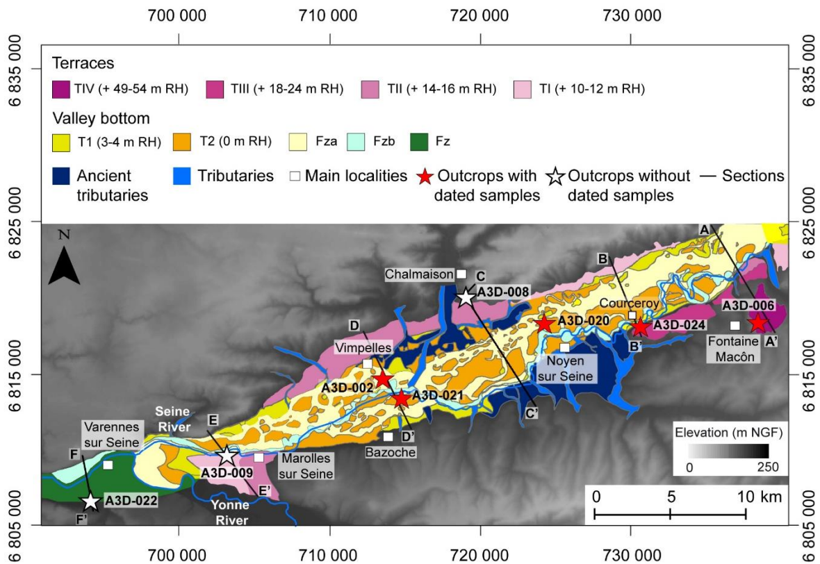
Figure 2.3. Homogenized geomorphological map within the Bassée alluvial plain (modified after Mégnien, 1965; Deleplancque et al., 2018), with location of the eight sites described and sampled for dating. Red stars represent outcrops with dated samples using the ESR/OSL dating methods. White stars represent outcrops without dated samples. Black lines represent topographic sections.
