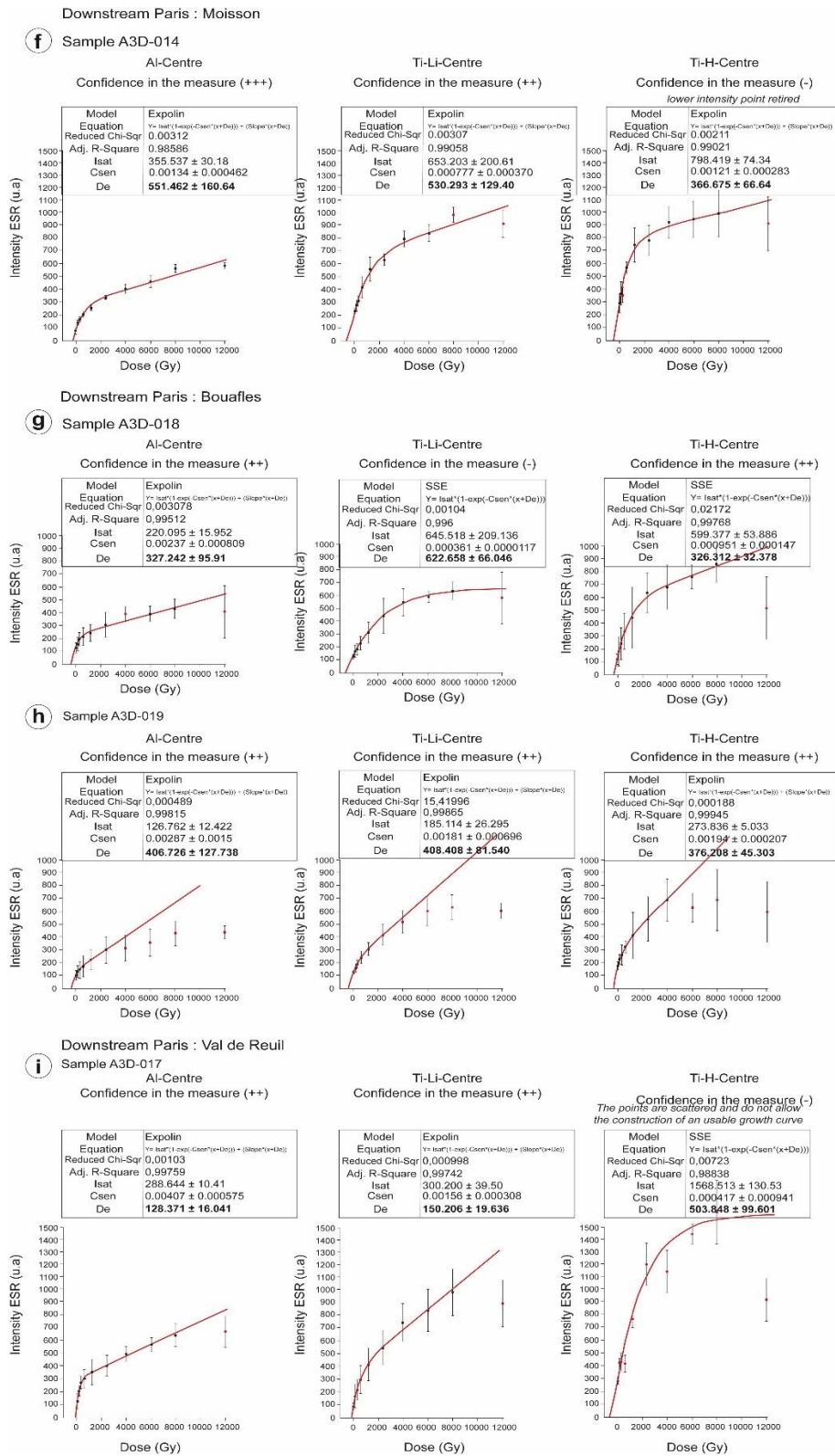
Figure C.3. Dose response curves were derived from the ESR signal of AI-centre, TiLi-centre and TiH-centre for samples located downstream of Paris at Moisson, Bouafles and Val-de-Reuil sites. Black points represent points used for final fitting, while red points represent data points removed for the fitting curve. Red line indicates the goodness-of-fit-curve found.
