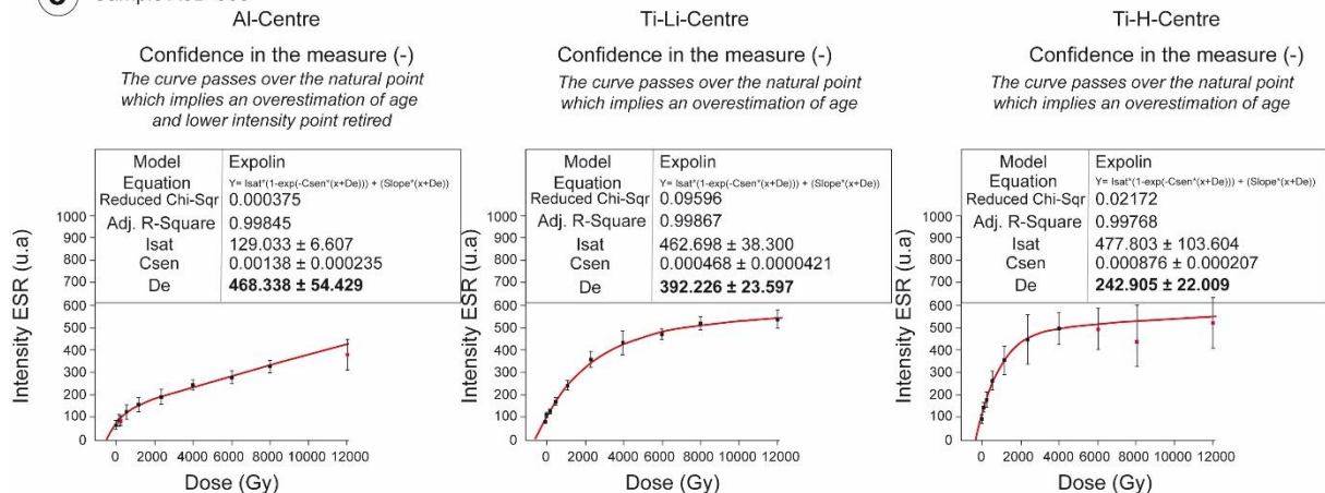
Figure C.2. Dose response curves were derived from the ESR signal of Al-centre, TiLi-centre and TiH-centre for samples located downstream of Paris, at Sandrancourt site, located in the Fyd terrace. Black points represent points used for final fitting, while red points represent data points removed for the fitting curve. Red line indicates the goodness-of-fit-curve found.
