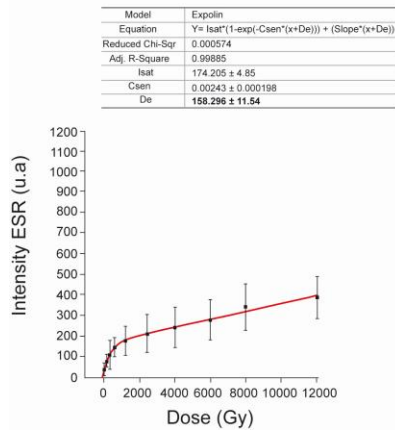
Figure C.1. Dose response curves were derived from the ESR signal of Al-centre, TiLi-centre and TiH-centre for samples located upstream of Paris. Black points represent points used for final fitting, while red points represent data points removed for the fitting curve. Red line indicates the goodness-of-fit-curve found.
