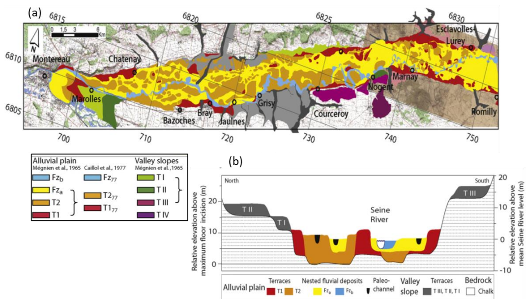
Figure 1.29. Upper Seine valley in the Montereau region, (a) Geomorphological map and (b) the cross-section of the Bassée alluvial plain (Deleplanque et al., 2018).
