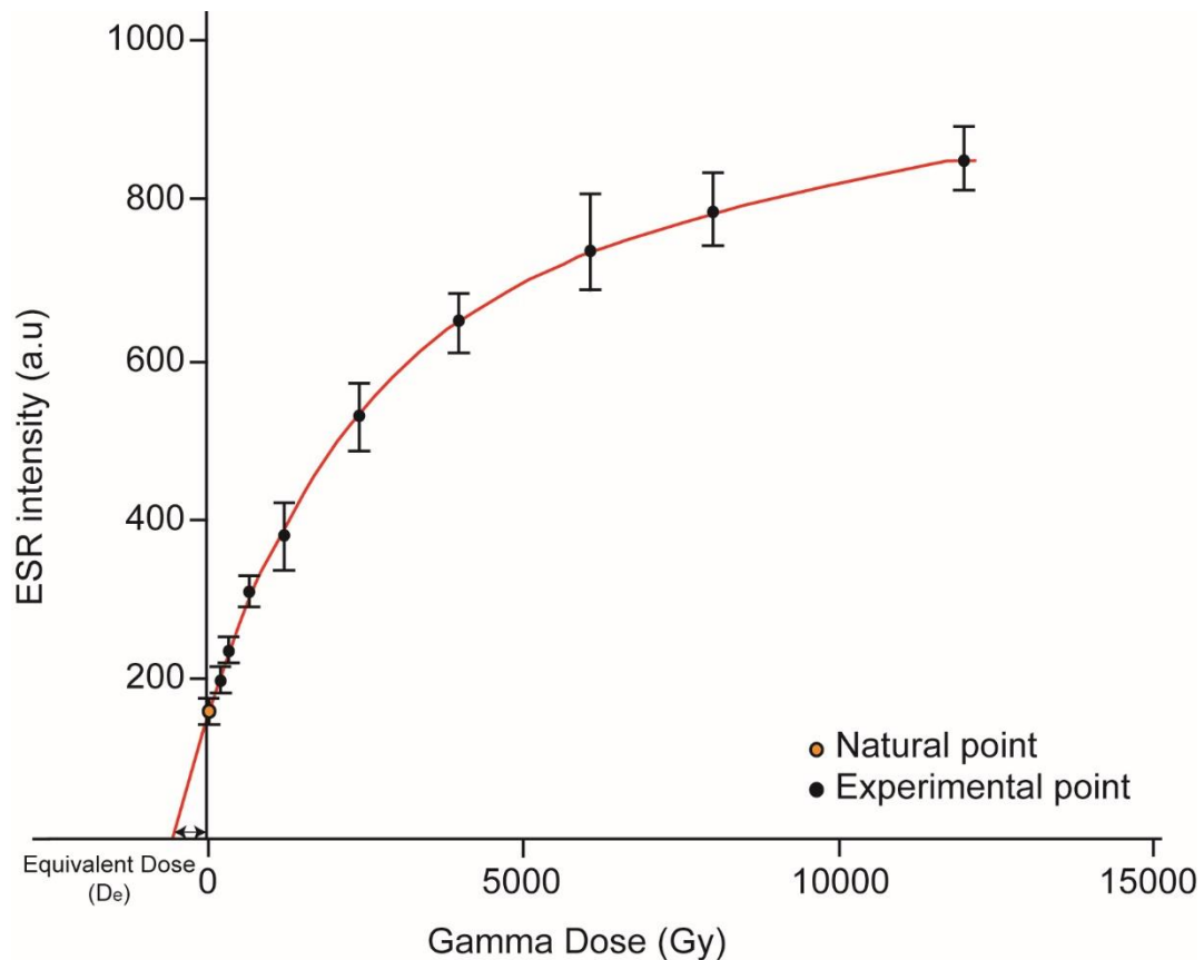
Figure 3.3. Determination of equivalent dose ( D_e ) using the additive method in sample A3D-015 using Al-centre.
