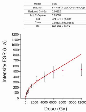
Figure C.1. Dose response curves were derived from the ESR signal of Al-centre, TiLi-centre and TiH-centre for samples located upstream of Paris. Black points represent points used for final fitting, while red points represent data points removed for the fitting curve. Red line indicates the goodness-of-fit-curve found.
