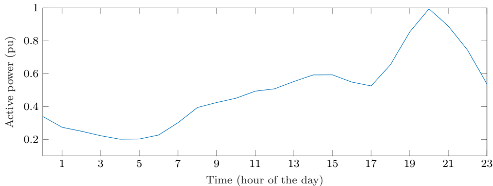
Figure 2.3: Profile of the net active power demand from CIGRE specifications[6].
