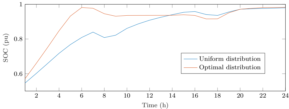
Figure 4.3: Comparison of mean SOC across the EVs population for different charging infrastructures with 20% higher demand than Fig 4.2.
