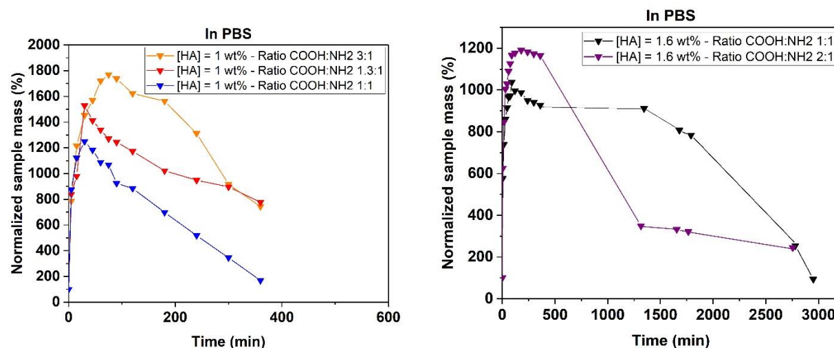
Figure 4.15. Normalized sample mass over time after immersion in PBS of 1 wt% HA (left) and 1.6 wt% HA (right) chemically crosslinked aerogels, prepared with different COOH:NH 2 molar ratios.
