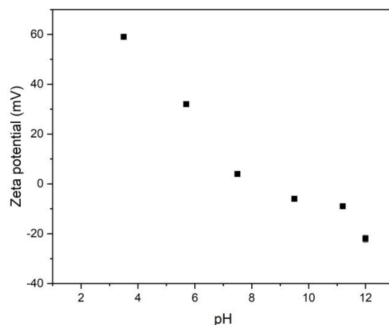
Figure 5.3. Zeta potential of nCh fiber suspensions between pH 3 and pH 12.
