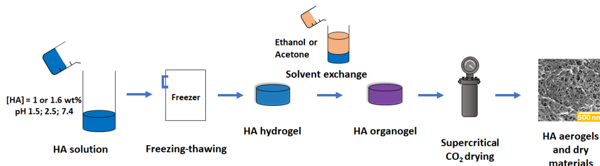
Figure 2.1. Schematic representation of the preparation of HA hydrogels via the freeze-thaw technique. Reprinted with permission from 4 . Copyright (2023) American Chemical Society.
