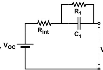
FIGURE 3.15 – First Order EC Model.
