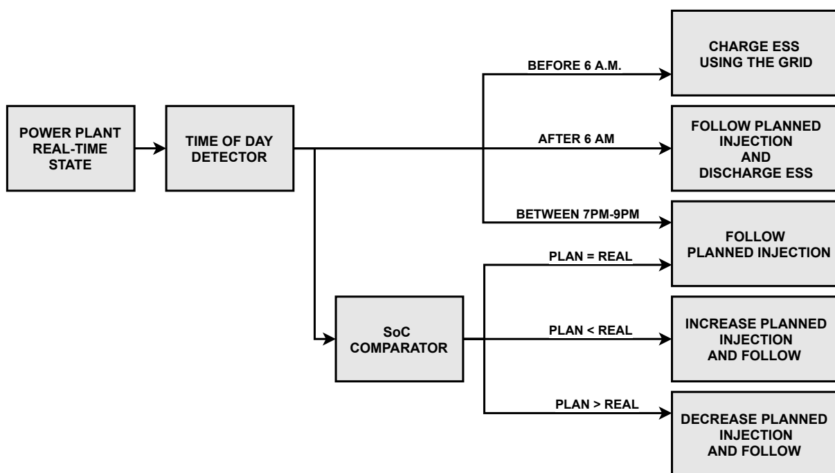
FIGURE 2.13 – Real-time logic used to decide whether to follow or to modify the scheduled objective power of the installation. EMS version from 14/09/2020.
