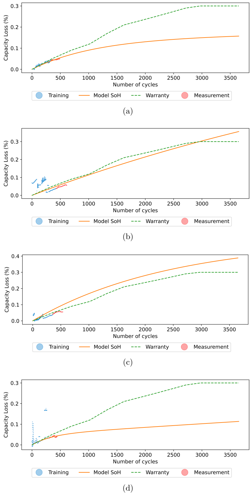
FIGURE 3.32 – Predicted SoH for LiBESS #4 - #7 in a 10-year horizon with 1-year of training data . The blue dots represent the training set, and the red dots the validation set : (a) LiBESS #4; (b) LiBESS #5; (c) LiBESS #6; (d) LiBESS #7.
