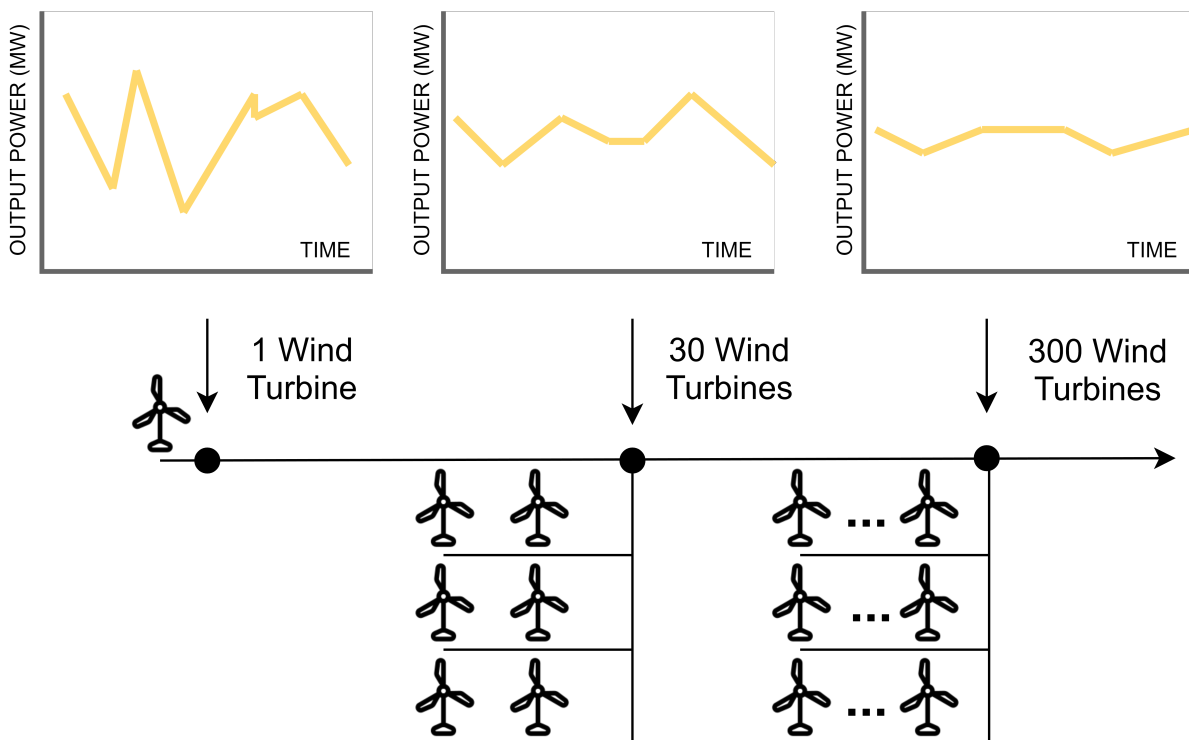
FIGURE 1.2 – Wind generation aggregation example. As the number of wind turbines considered increases (left to right), the power injection to the grid (yellow line) seen at the PCC has less intermittence and variance. Adapted from : [9].
