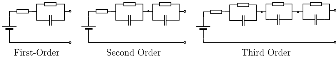
FIGURE 1.8 – RC equivalent circuits of a battery cell
