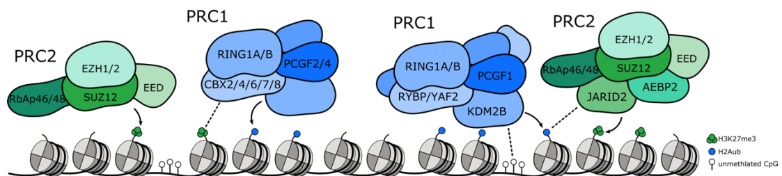
Figure 3. Polycomb repressive complexes coordinate transcriptional silencing.
